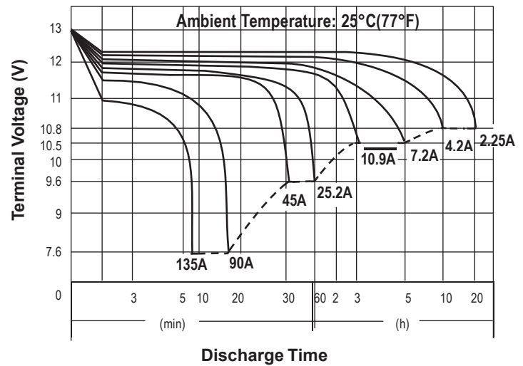
Discharge Characteristics
